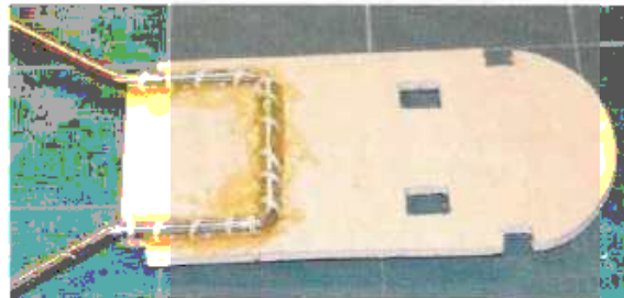
Bind and epoxy the planowire undercarriage to former F1.
